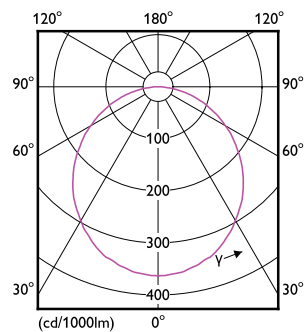
Downlight 59466 MESON 150 65K WH Recessed-LDD
